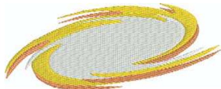
39 - Milky Way Ellipse
